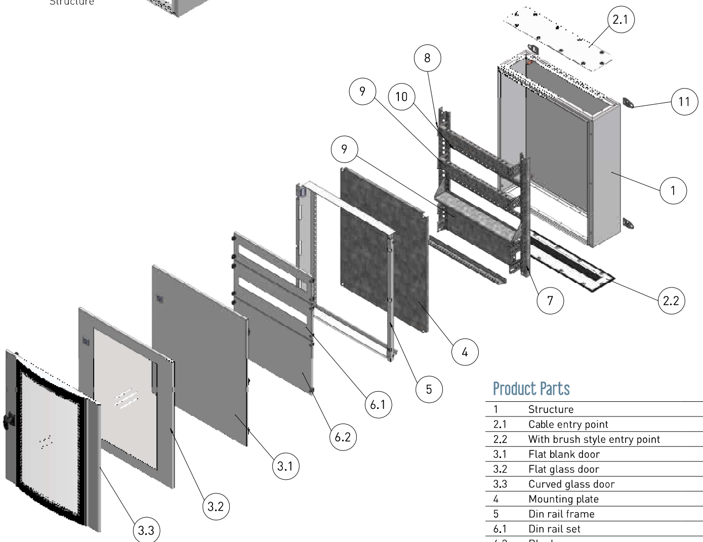
Monoblock Structure
