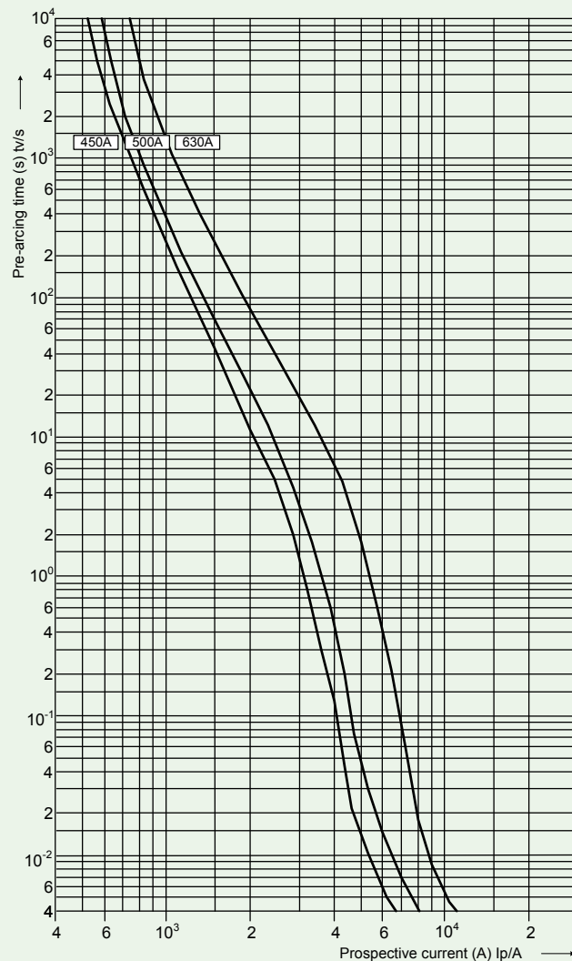
gPV, PV(gR) 1100V t-l characteristics
