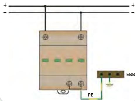
V configuration ETITEC S B-PV U/I_{imp}
