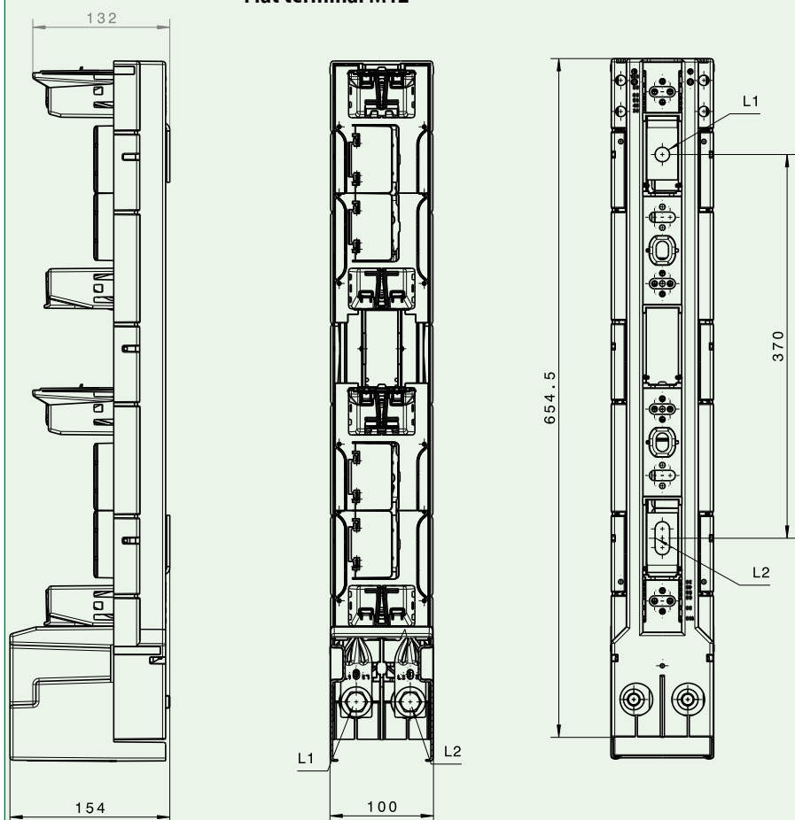
Flat terminal M12
