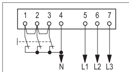
3-phase line with insulated
