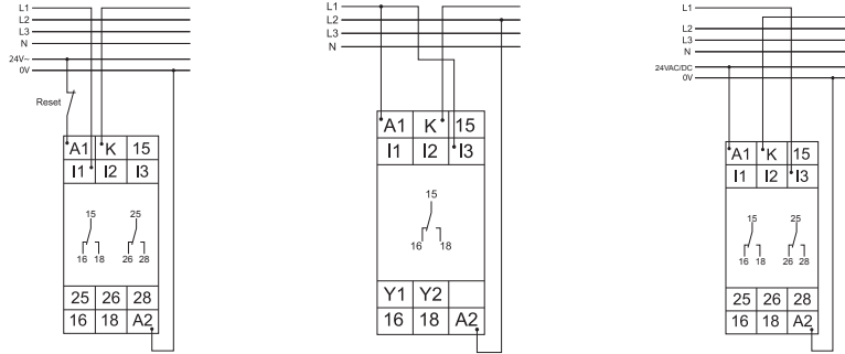
Measuring range 20mA AC/DC, supply voltage: 24V AC/DC Measuring range 5A AC/DC with Powermodule 400V AC Measuring range 2A AC/DC, supply voltage: 24V AC/DC
