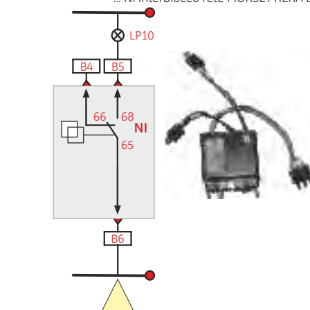
... NI Network Interlock BLOCK B ... NI Network Interlock BLOCK B ... NI interblocco rete MORSETTIERA B
