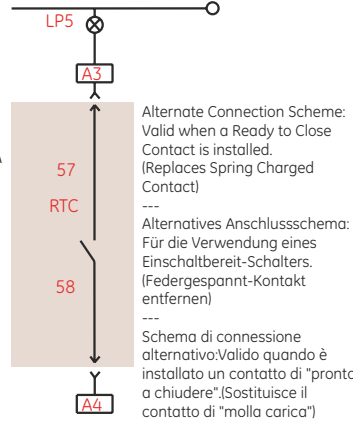
Connection scheme RTC (BLOCK A) Anschlüsse RTC (BLOCK A) Schema connessione RTC (Morsettiere A)
